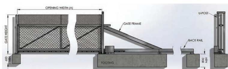
Cantilever Sliding Gate
