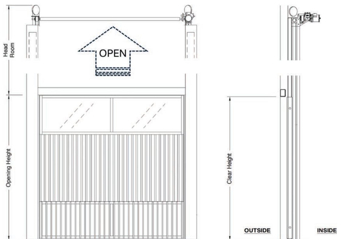
Elevation (FRONT VIEW)
